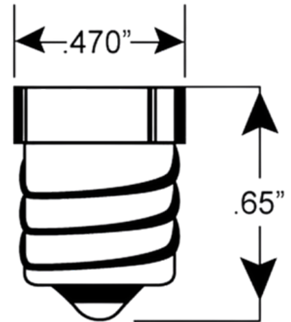
C7/Candelabra Base (E12)
